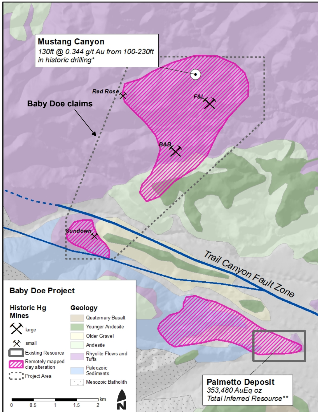
Figure 2: Geologic map of Baby Doe project area showing areas of alteration, mercury occurrences and adjacent, outcropping gold systems
