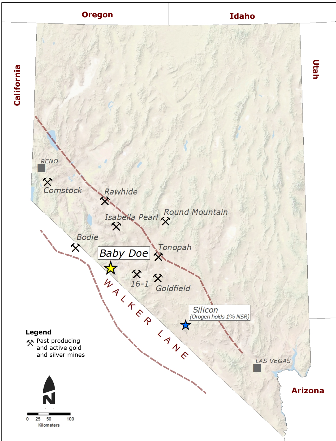
Figure 1: Location map showing the Baby Doe project located in the White Mountains, Esmeralda county, Nevada
